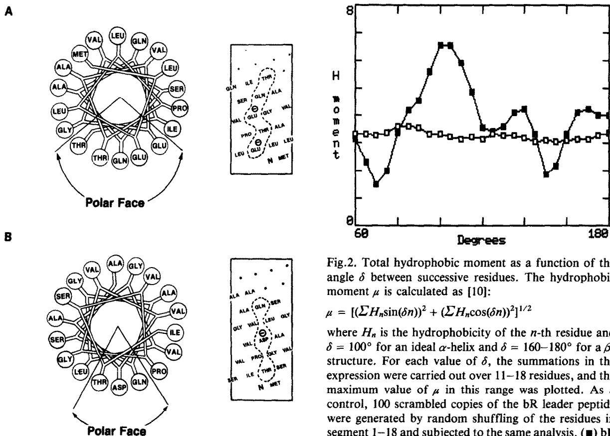
Fig.1. Helical projections of the bacteriorhodopsin (A) (bR 1-18) and halorhodopsin (B) (hR 3-20) leader peptides. The polar patches are shaded. Bacteriorhodopsin is cleaved preferentially after residue 13, halorhodopsin after residue 21.
